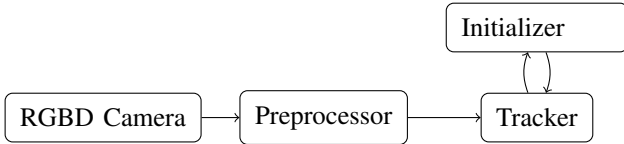
Fig. 4: Tracking pipeline.
