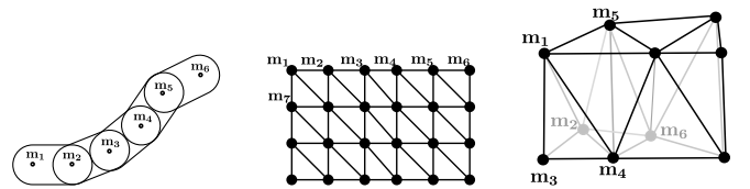
Fig. 2: Physical model for three classes of deformable object: (a) one-dimensional object, which we model as a chain, (b) two-dimensional object, which we model as a mass-spring system on a triangular mesh, (c) three-dimensional object, which we model as a mass-spring system on a tetrahedral mesh.
